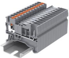
TP2.5-2-1-GY
